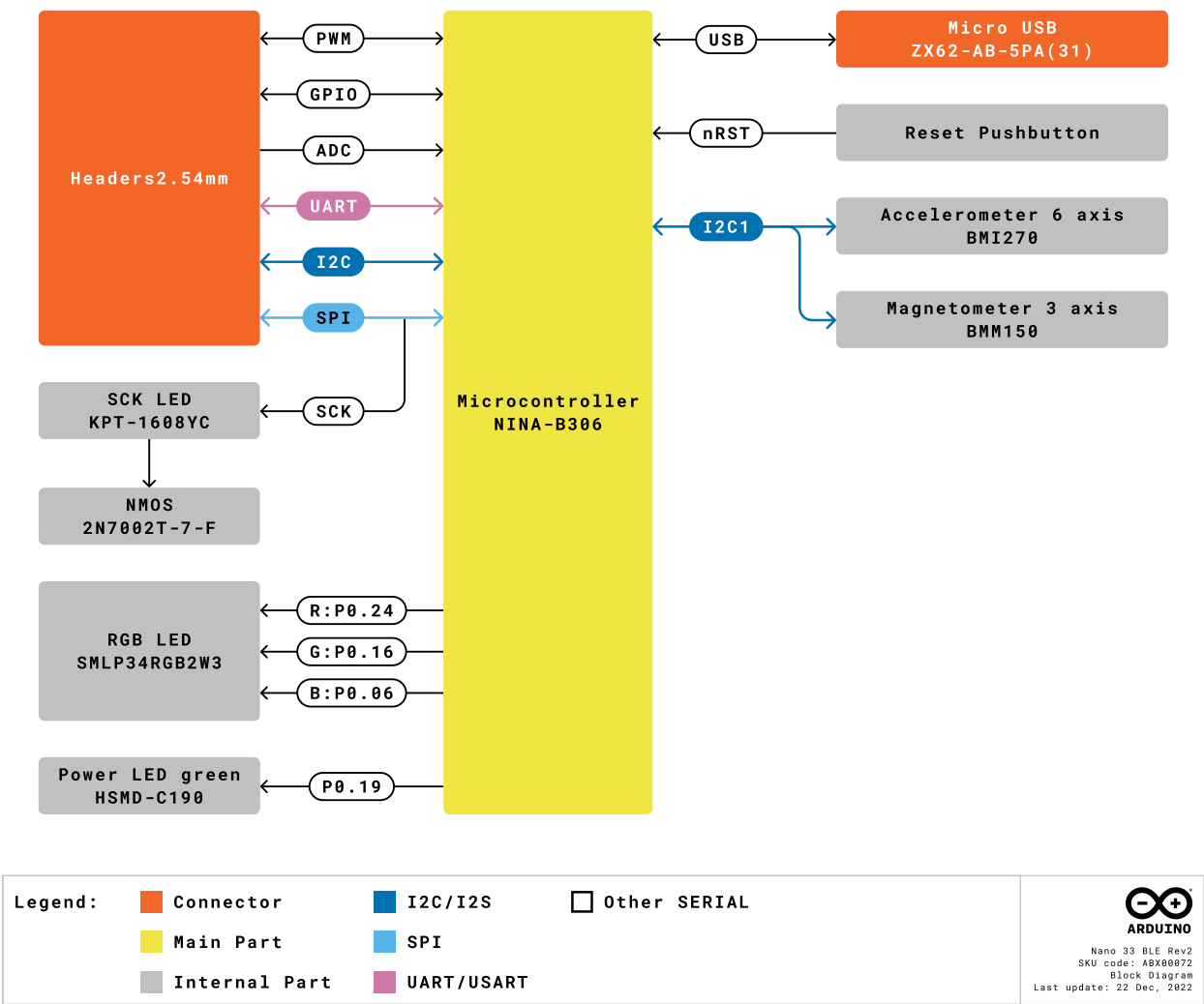
Block Diagram
